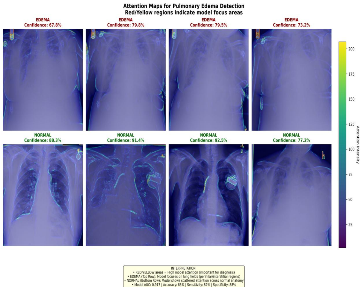
Figure 4. 6 Attention Maps
